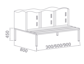
bancos/bancos
